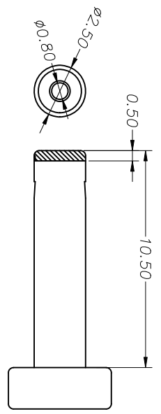
Ø2.5mm 2 POLE PLUG DETAIL DRAWING
