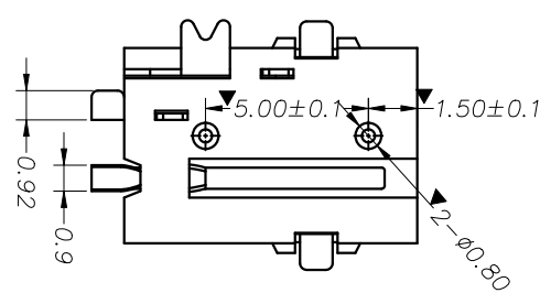
Ø2.5mm 2 POLE PLUG DETAIL DRAWING
