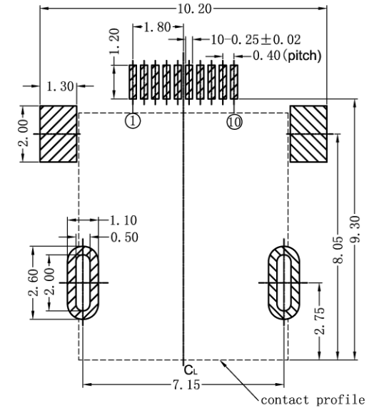
Recommended P.C.B Layout (Top Side) Tolerance = ± 0.05
