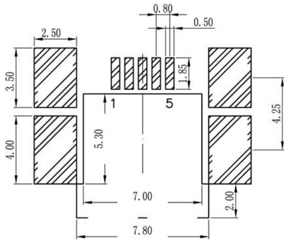
P.C.B LAYOUT TOLERANCE: \pm 0.05
